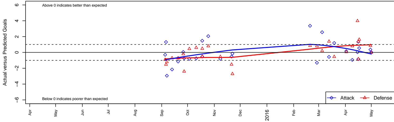
NPSA Titans Navy G01 Dots are actual minus expected GF (blue circles) and GA (red triangles). Blue line is smoothed change in attack strength. Red is smoothed change in defense strength.
